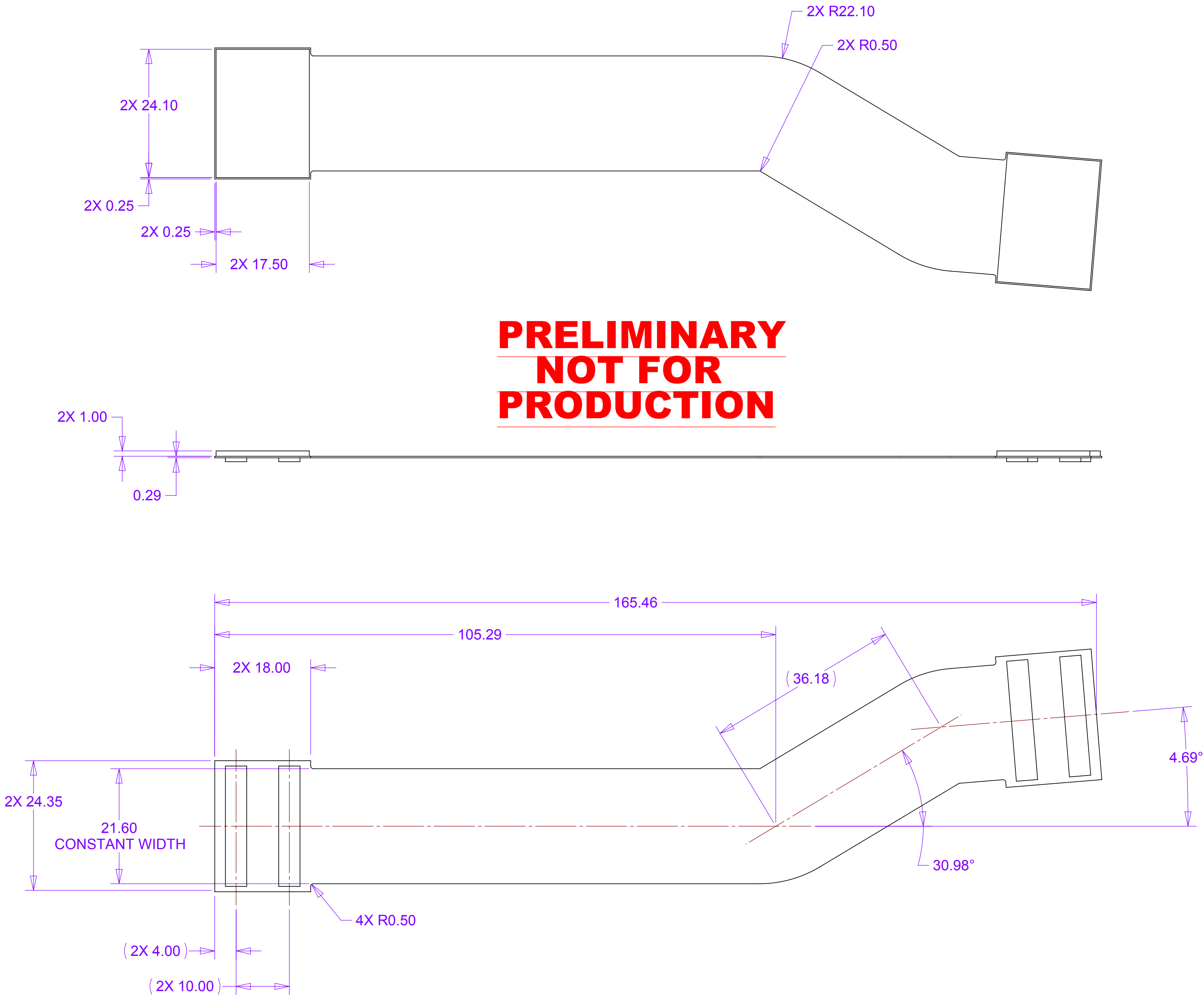
FLAT PATTERN VIEW
